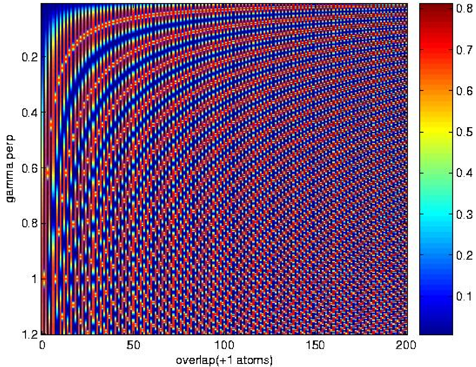
T(gamma perp, overlap) at Fermi-level
