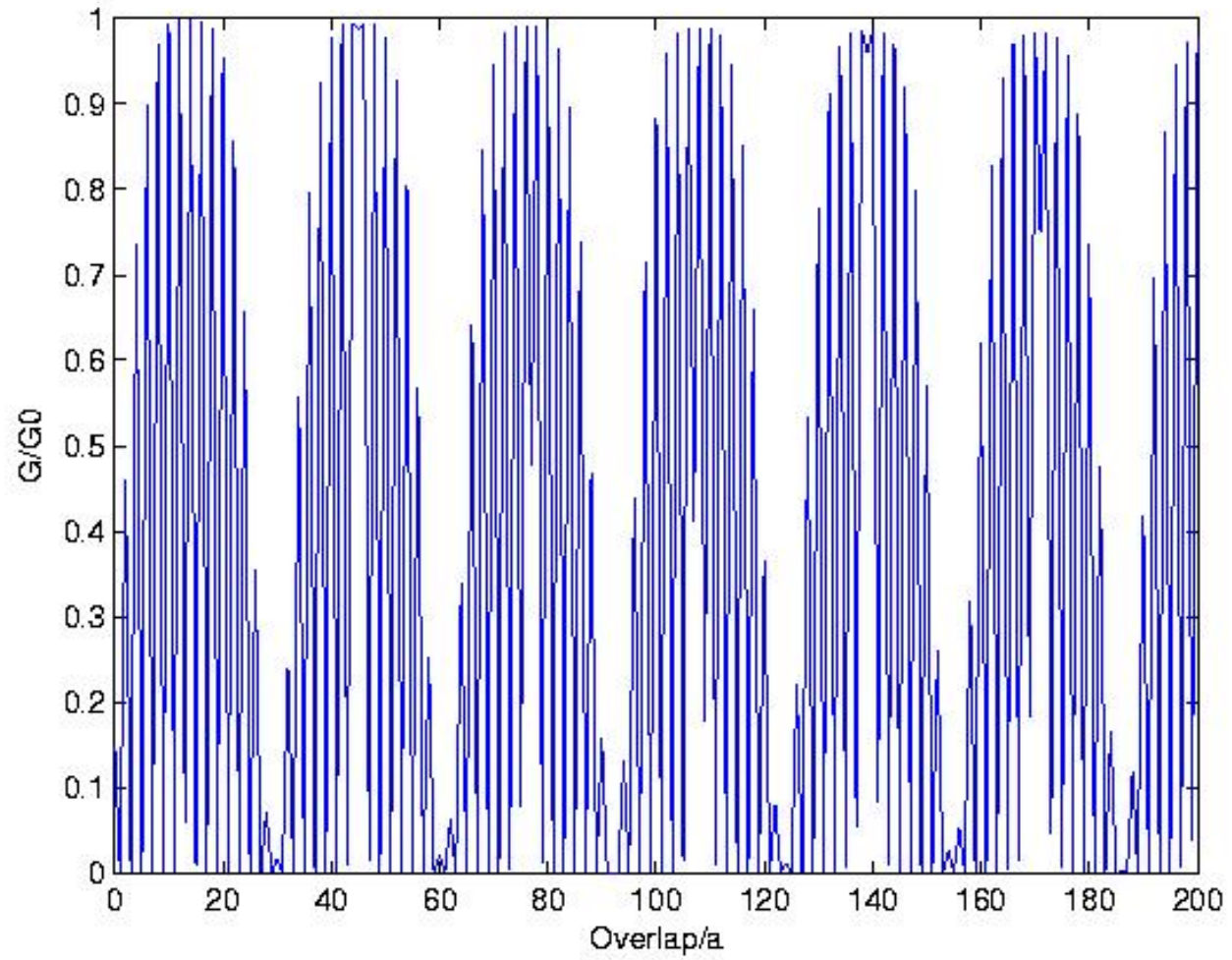
G(Overlap) at the Fermi-level gamma perp=0,2, gamma parallel=1
